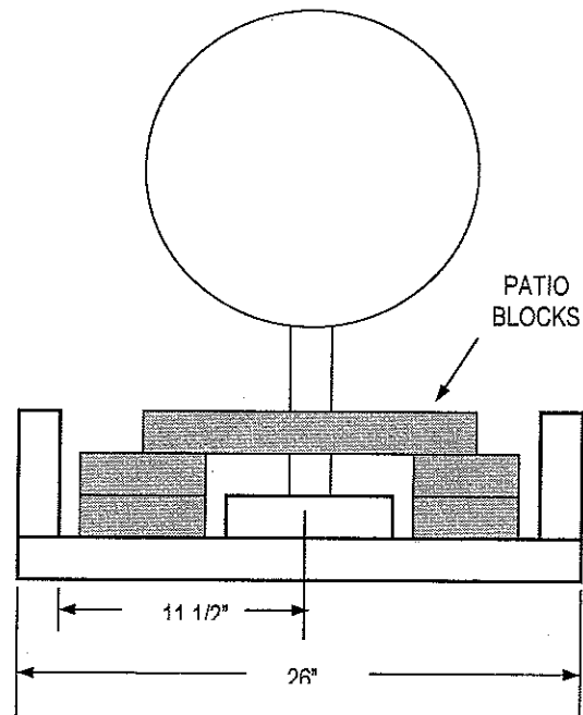
PATIO BLOCK PLACEMENT
